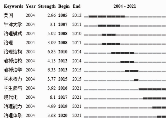
Top 12 Keywords with the Strongest Citation Bursts
